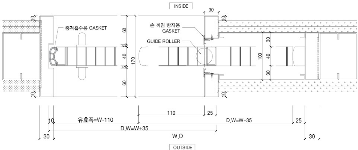
HORIZONTAL SECTION
