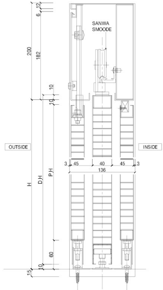
VERTICAL SECTION
