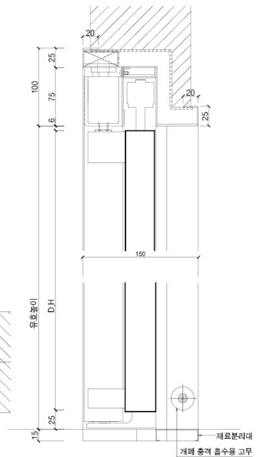
VERTICAL SECTION
