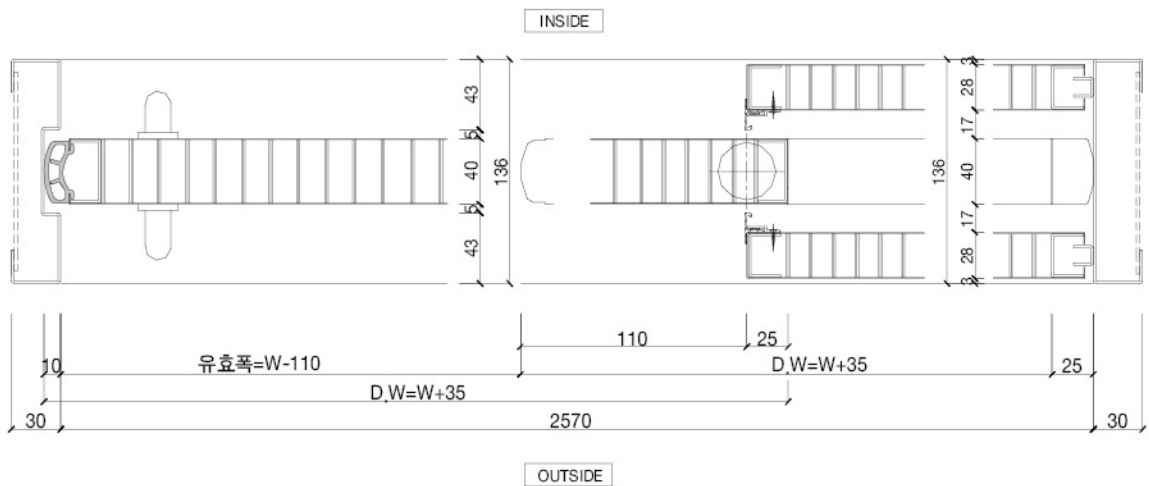
HORIZONTAL SECTION
