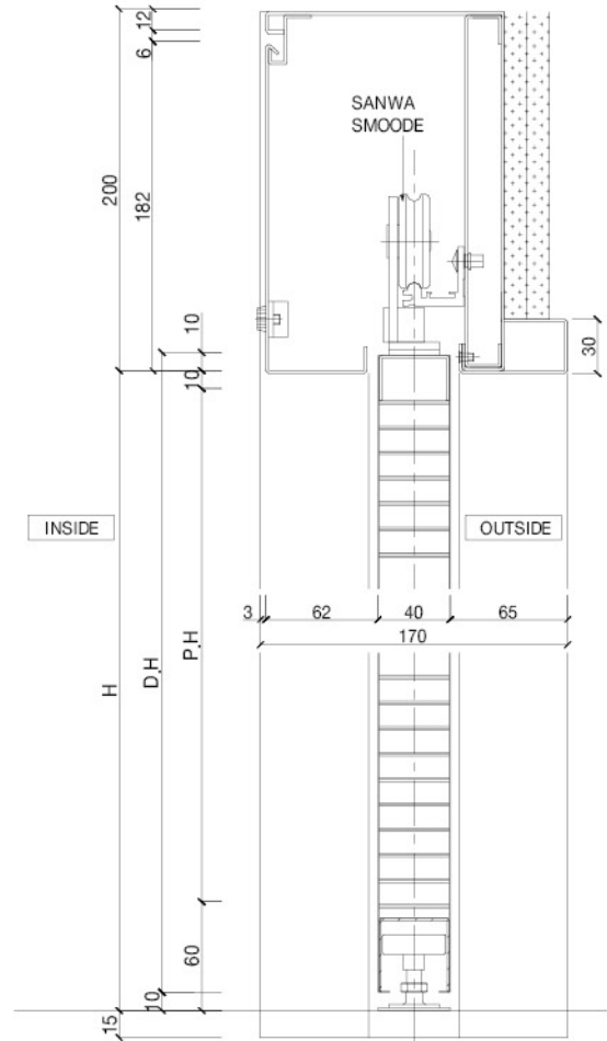
VERTICAL SECTION
